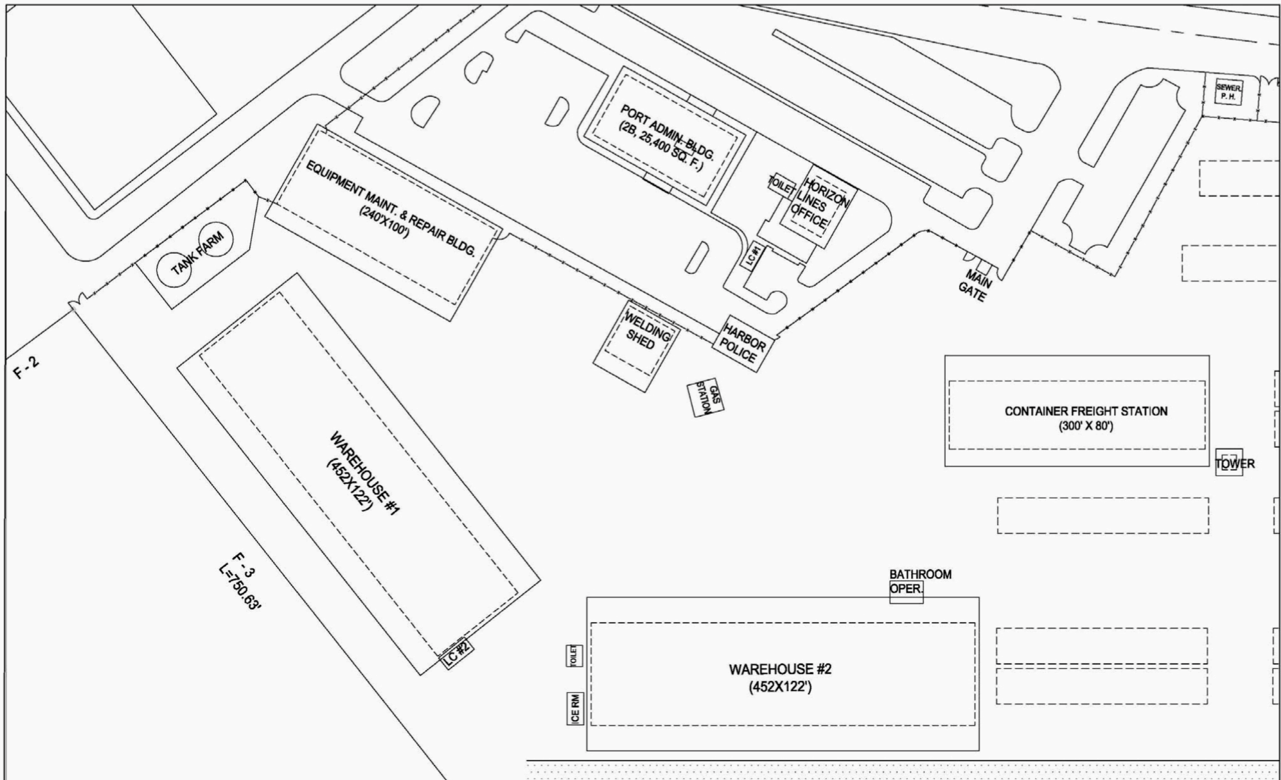
Figure 2.3-2 Cargo Terminal Area Buildings Structures
