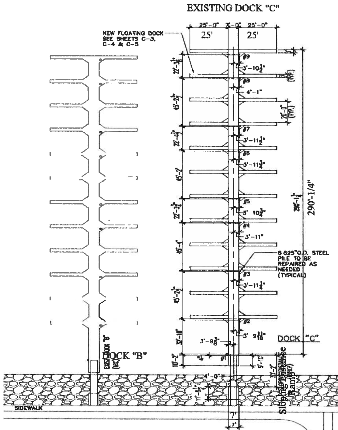
EXISTING DOCK "C" FLOATING DOCK CONFIGURATION (TYPICAL TO DOCK "B")
